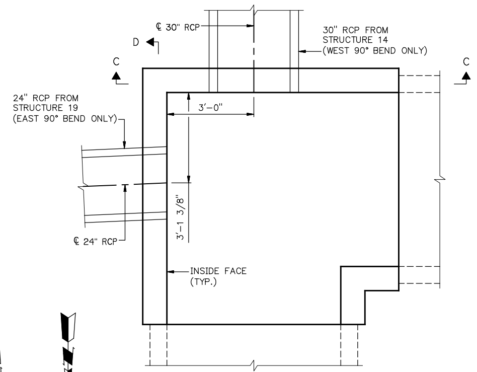
RCP STUB PLAN
