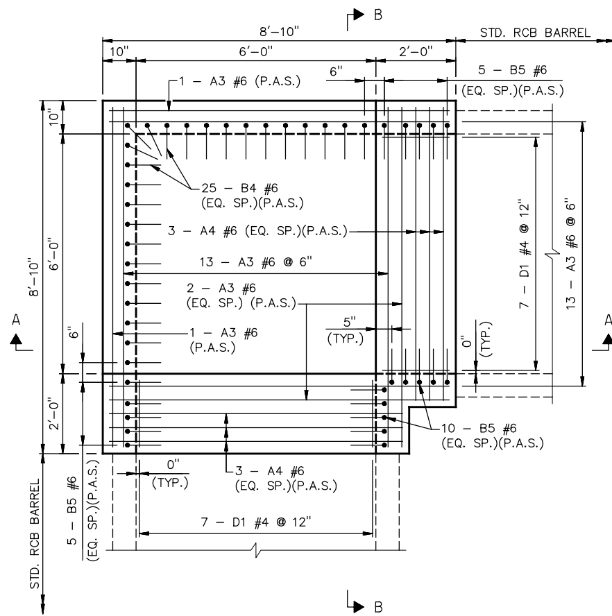
TOP SLAB TOP REINFORCING MAT PLAN
