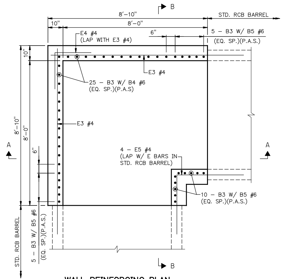
WALL REINFORCING PLAN
