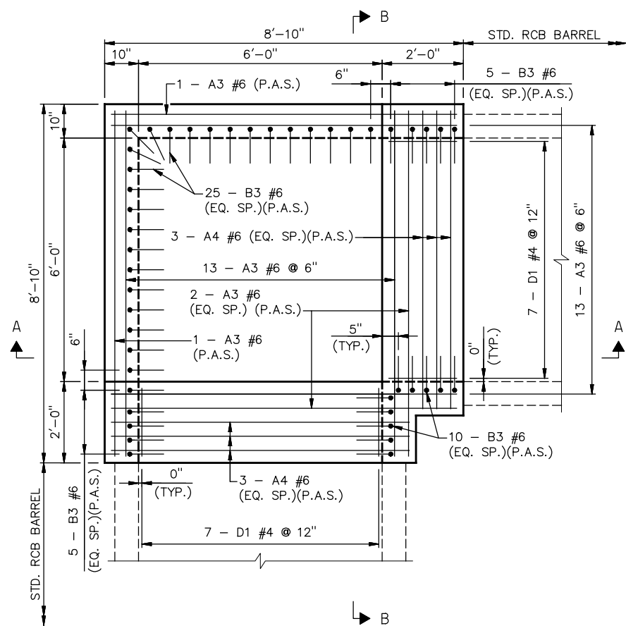
BOTTOM SLAB BOTTOM REINFORCING MAT PLAN
