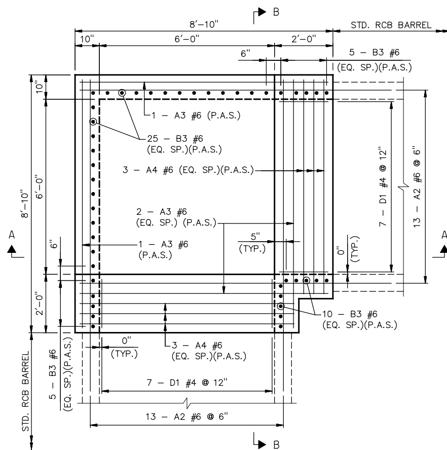
BOTTOM SLAB TOP REINFORCING MAT PLAN
