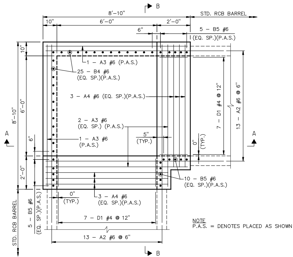
TOP SLAB BOTTOM REINFORCING MAT PLAN
